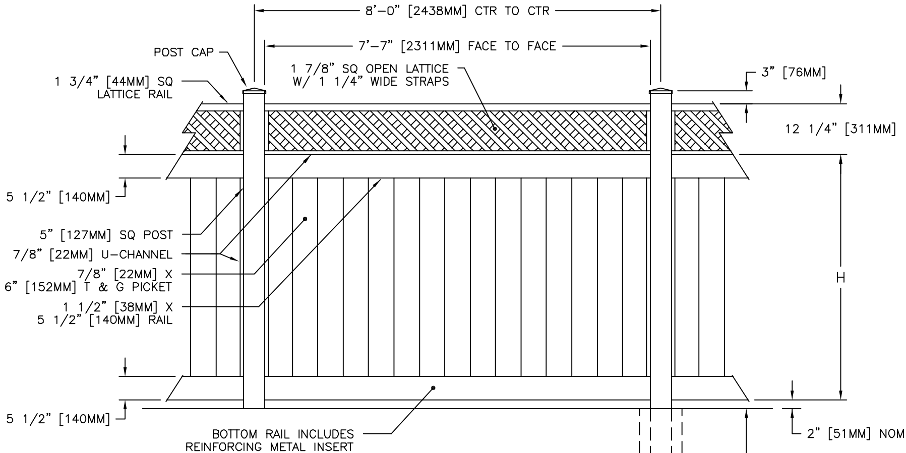
FENCE SECTION ELEVATION
