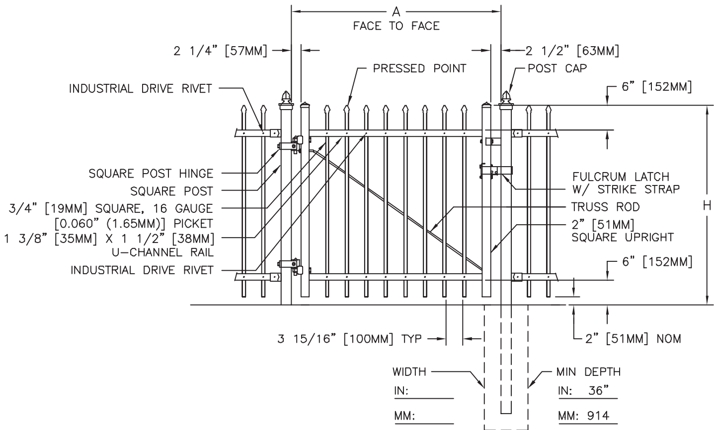
GATE ELEVATION
