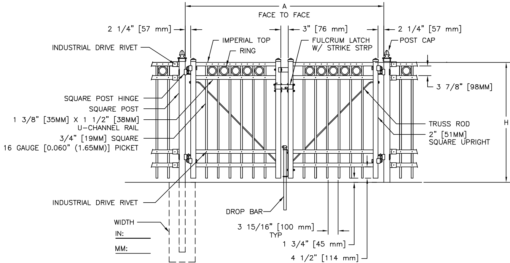
GATE ELEVATION
