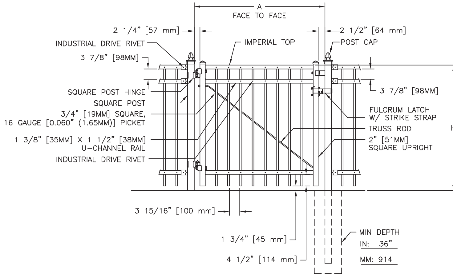
GATE ELEVATION
