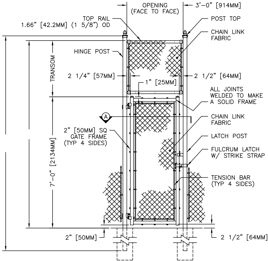
GATE ELEVATION
