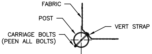
SECTION A TYP CORNER POST (NTS)
