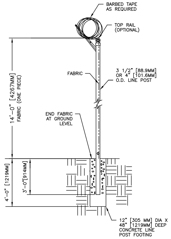
END VIEW DETAIL (NOT TO SCALE)
