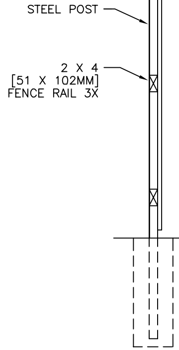
END VIEW
